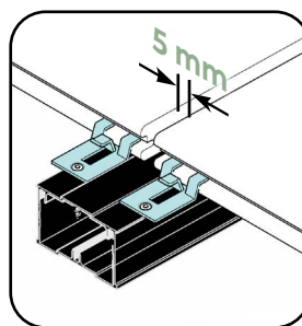
Lambourde aluminium Silvadec® + clips simples
