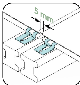
Doubles lambourdes composite + clips simples
